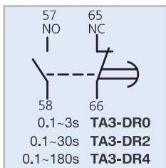
Off Delay Timer Block (Front mounted) TA3-DR2
