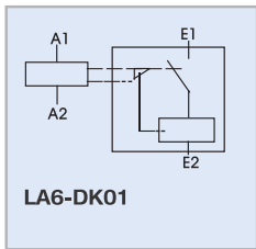
Latch Add-on Block (Front mounted) LA6-DK01
