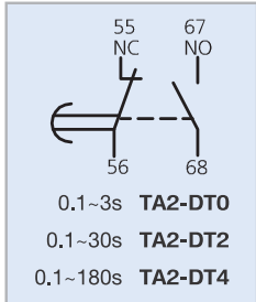
On Delay Timer Block (Front mounted) TA2-DT2
